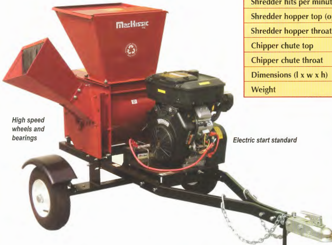
71 lb. rotor/flywheel assembly with 48 free-swinging hammers
